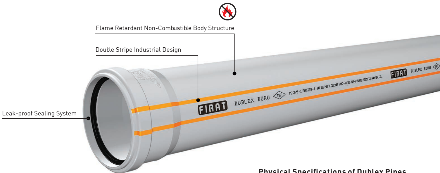
Physical Specifications of Dublex Pipes
